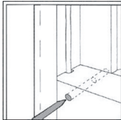
Nails can be used to “pin” a double-hung wood window. Do not use on vinyl or metal windows.
